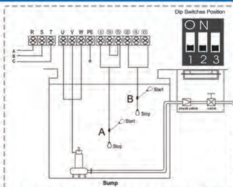
Wiring diagram for one sewage pump
