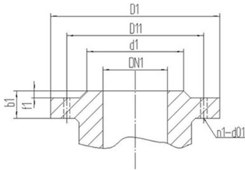
Inlet Flange Data
